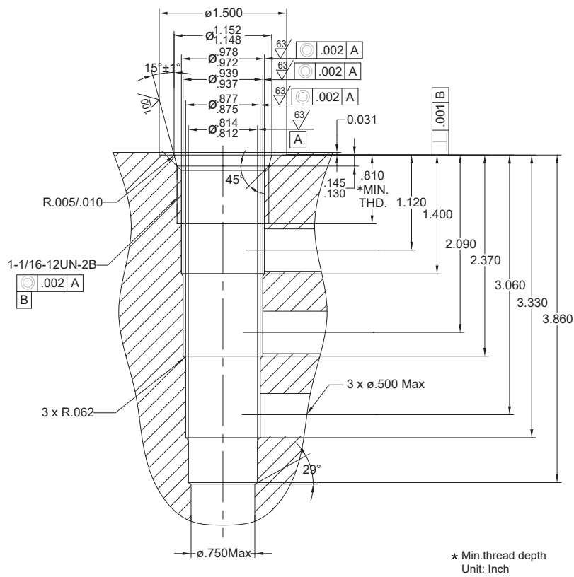
CAVITY:12-4
