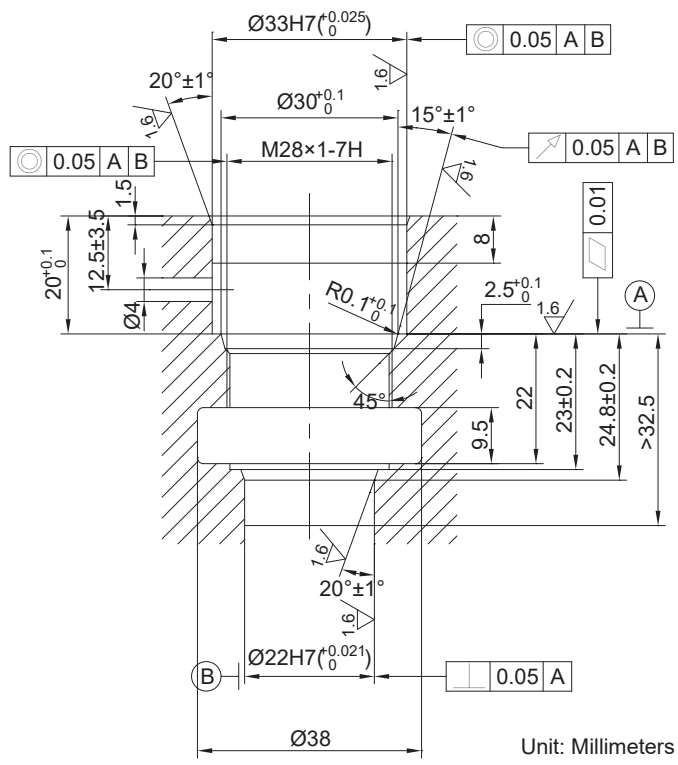
CAVITY:Rexroth-HC
