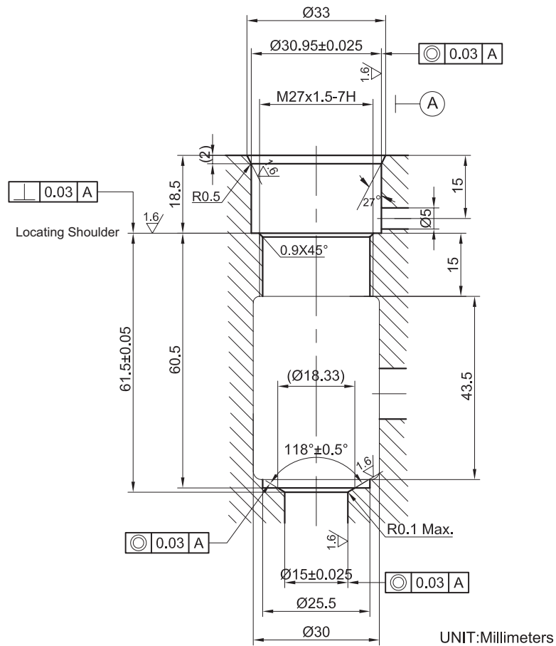
CAVITY:12M-3
