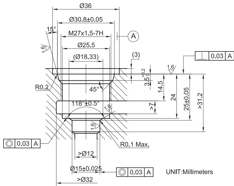
CAVITY:12M-2
