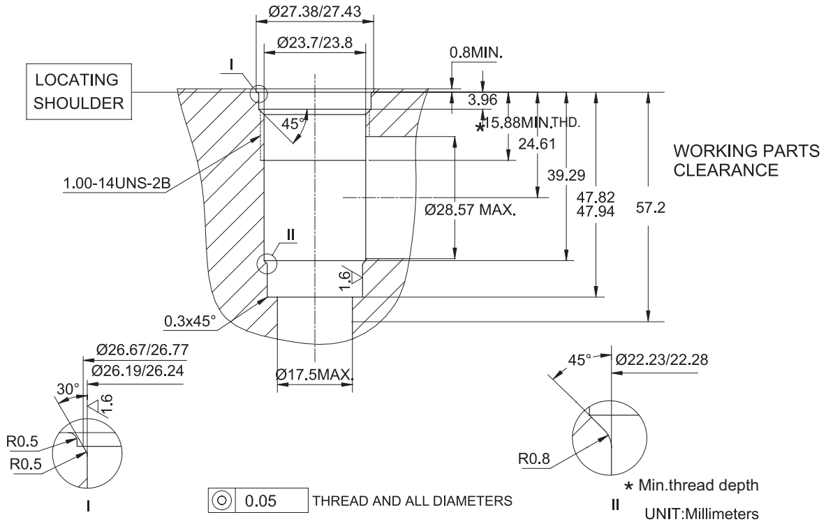
CAVITY:SUN T-3A
