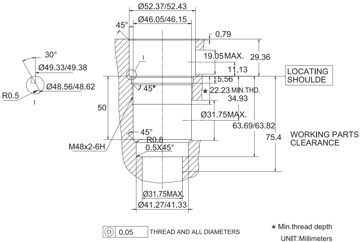
CAVITY:SUN T-19A
